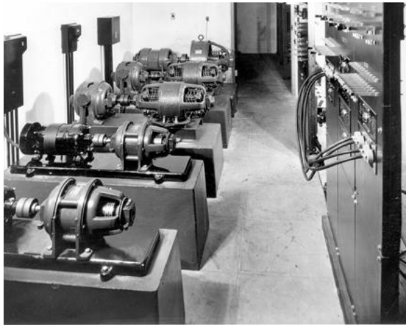
1928 Interlock generators and patch panel
