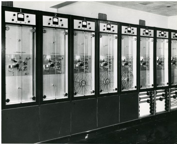
8-tracks of optical dubbers in late 1940s. The three right machines show loop cabinets for background effects such as rain. The right image shows how optical dubbers were simply updated with mag heads/electronics and continued to be used as 3-track mag dubbers. Optical dubbers like these, and even earlier machines from the late 1930s were still being used as mag machines in the 1970s due to the quality of their original construction. Photos: Endpoint museum collection.
