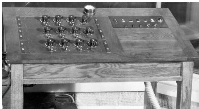
1928 Modular Western Electric mixer capable of any number of inputs and groups by adding panels as desired. By March 1928 they were already specifying nine inputs and two group outputs. The version on right is similar but uses three output groups (right-most knob on each of the panels). Photo: Endpoint museum collection
